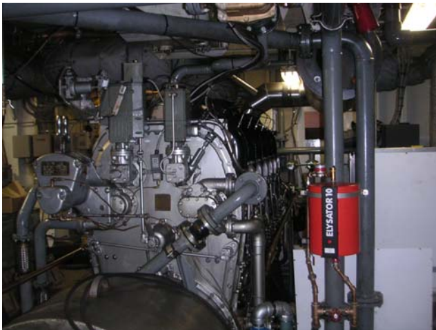
ELYSATOR 10 - Cleveland Diesel Cooling Circuit
